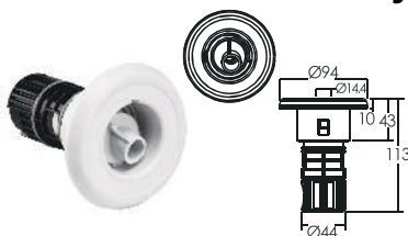
Smooth Face Swirl Jet
